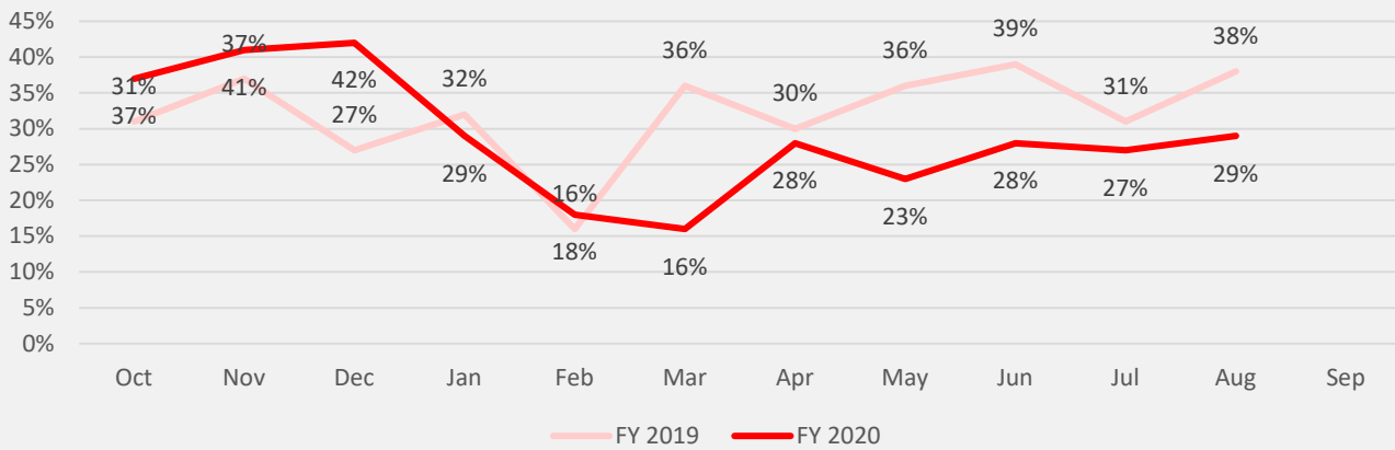
Overlapping Calls
