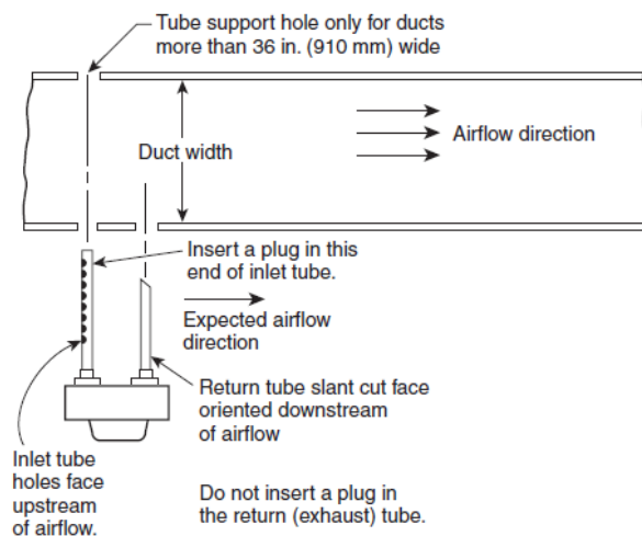
FIGURE A.17.7.5.5.2(b) Inlet Tube Orientation.
