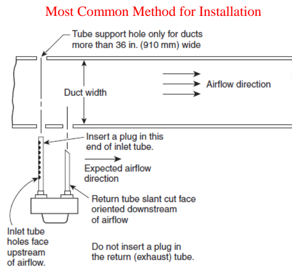
FIGURE A.17.7.5.5.2(b) Inlet Tube Orientation.
